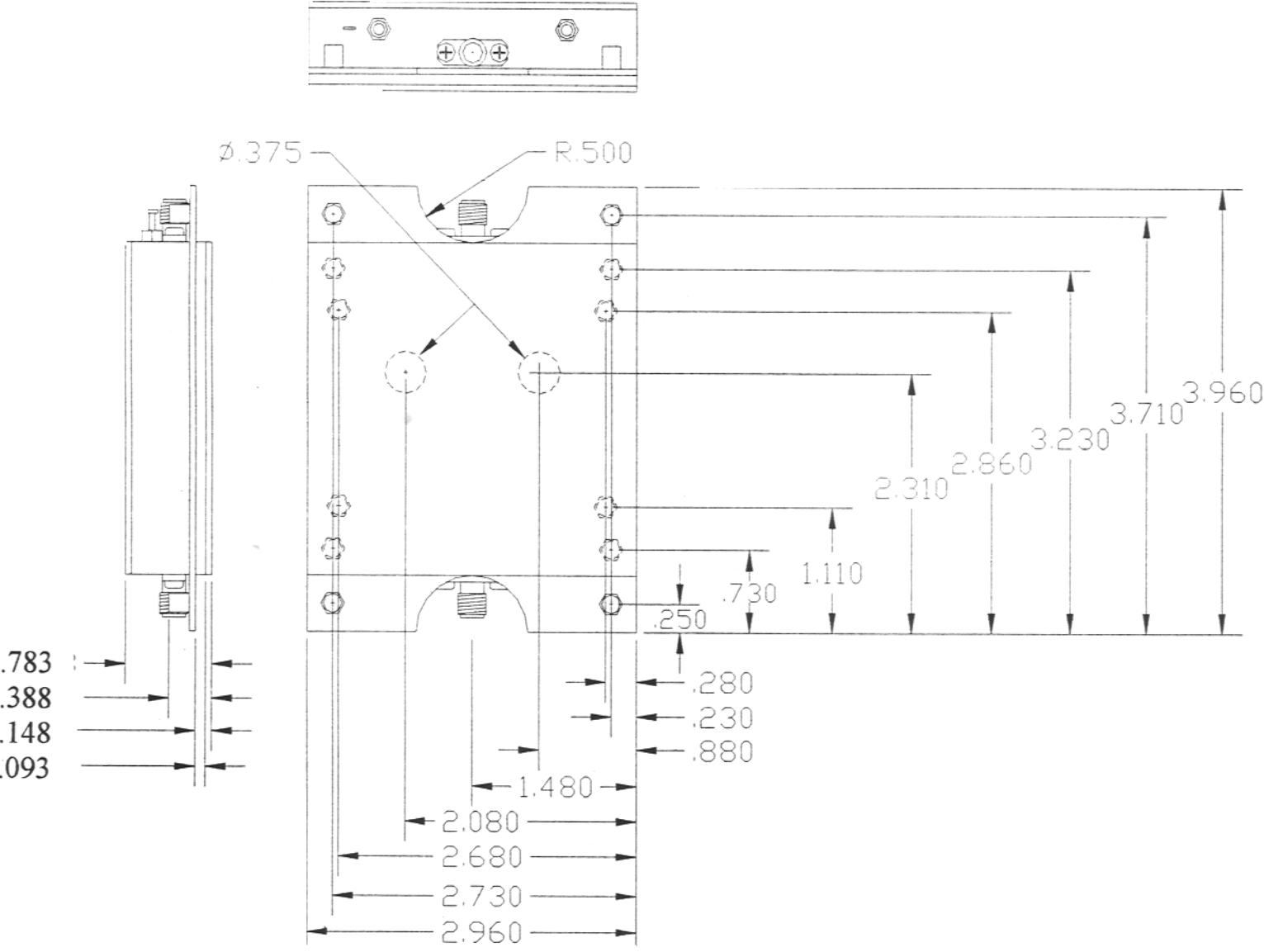
Case Dimensions (in inches)
